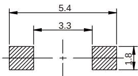
Land Pattern: [mm]
